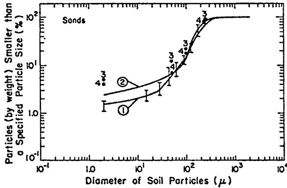
Fig. 8. Summation percent curves for sands (numbers in figure refer to soil sample numbers in Table II).
