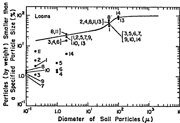
Fig. 10. Summation percent curves for loams (numbers in figure refer to soil sample numbers in Table II).
